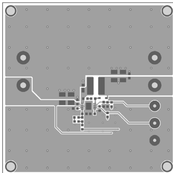
Figure 2 – Top Layer
