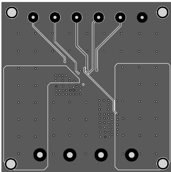
Figure 3: Inner Layer 2
