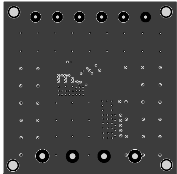
Figure 2: Inner Layer 1
