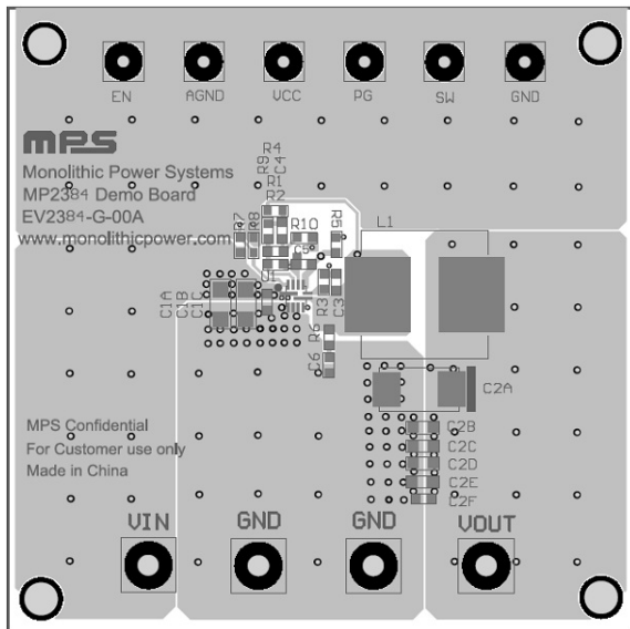
Figure 1: Top Layer and Silk
