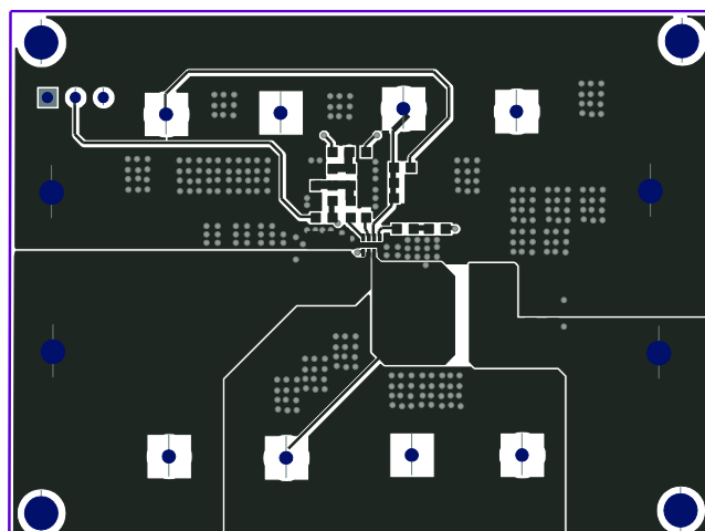
Figure 3: Top Layer
