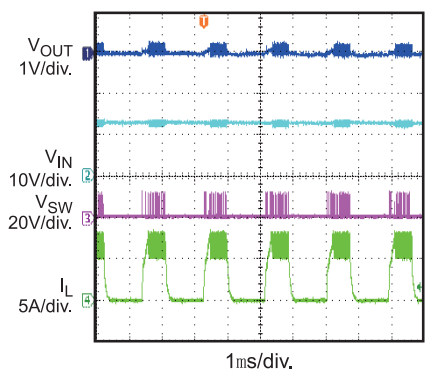
Short-Circuit Steady
