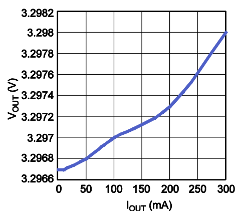
V_{OUT} vs. I_{OUT} V_{IN}=4.3V
