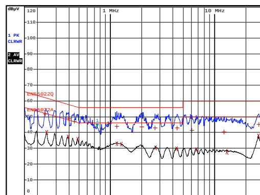
Conducted EMI Live Wire
