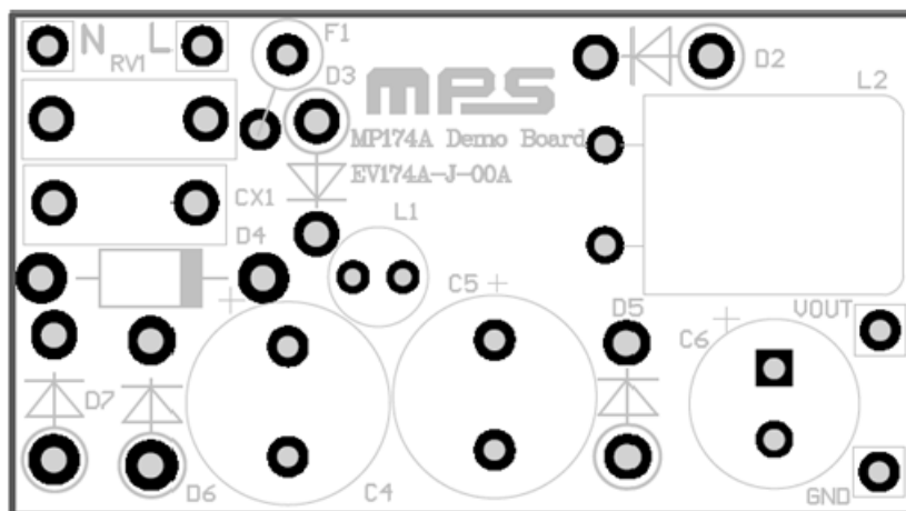
Figure 2: Top Layer
