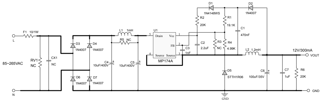
Figure 1: Schematic
