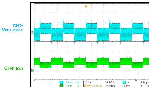
Load Transient
