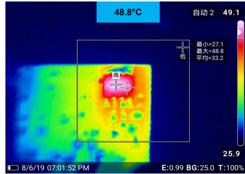
Thermal V_{IN}=265V_{AC}
