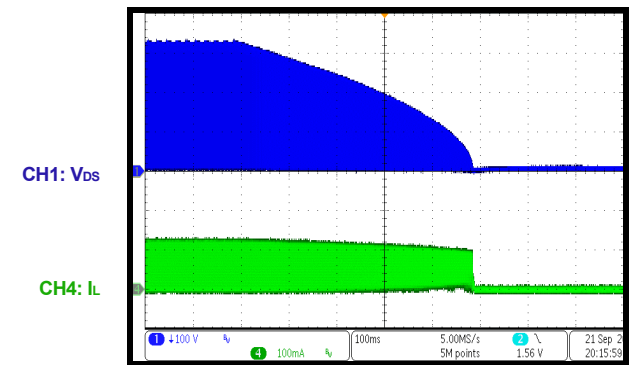
Shut-down
