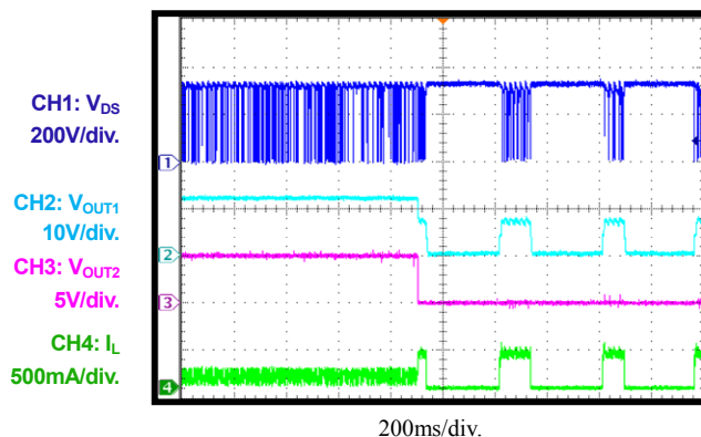
V_{OUT2} Short Circuit
