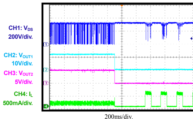
V_{OUT1} Short Circuit
