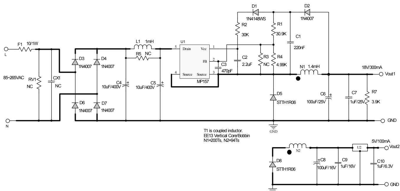
Figure 1—Schematic
