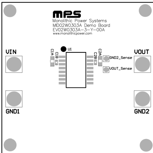
Figure 1: Top Silk
