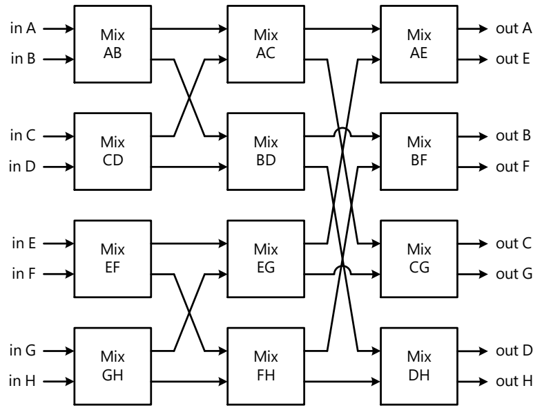
Figure 19. Butterfly mixer
