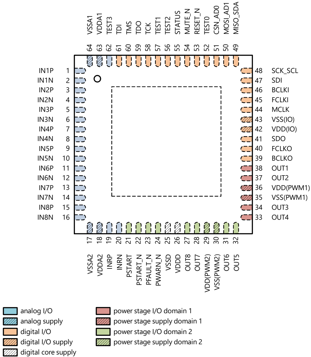
Figure 2. AX5689C top view
