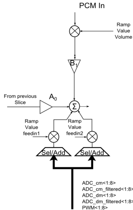
Figure 16. Feed-in filter
