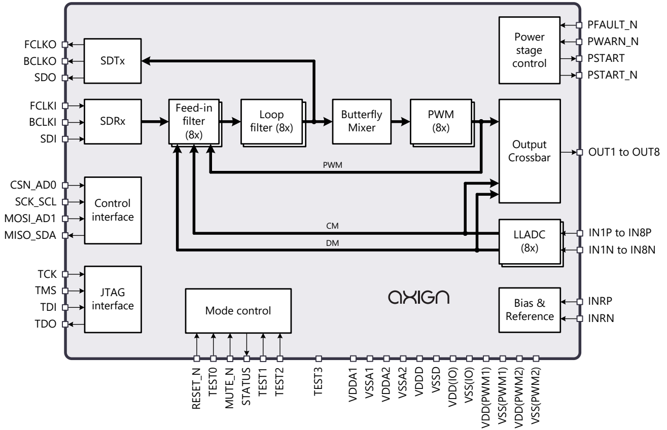
Figure 1. Block diagram AX5689C
