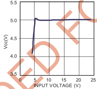
VCC Regulator Line Regulation
