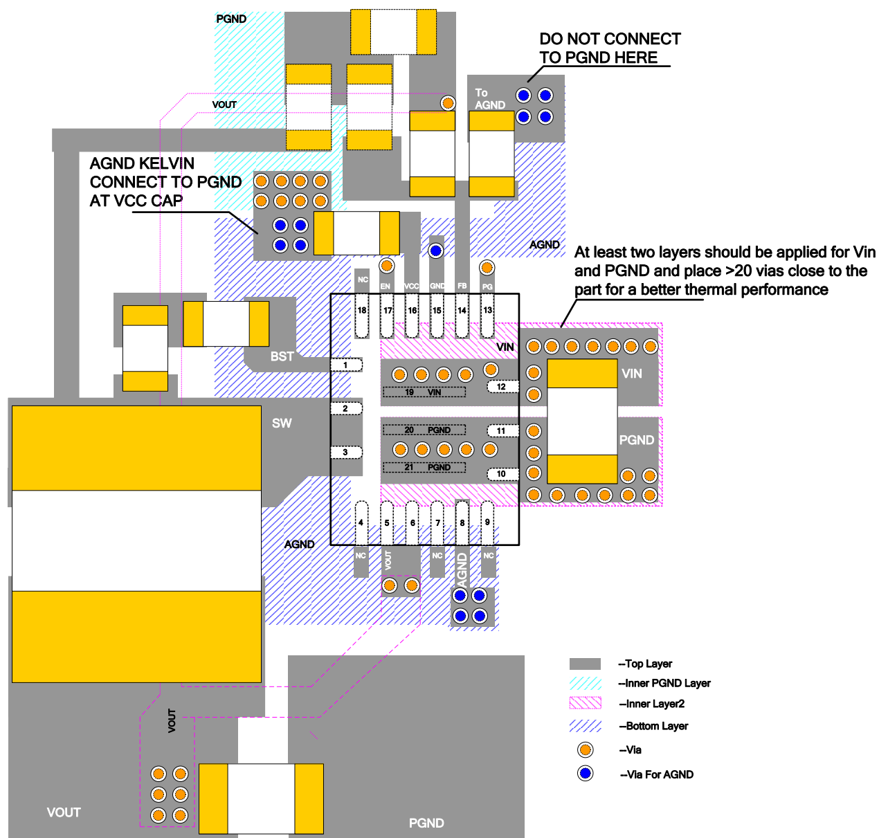
Figure 13—Recommend Layout
