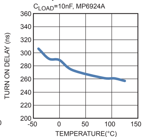
Turn-On Delay vs. Temperature
