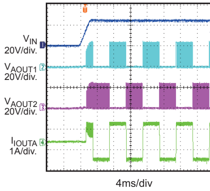
Power Ramp Up-Full Step
