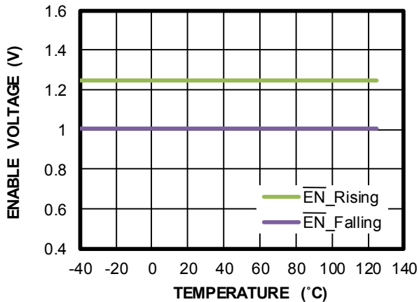
\overline{\text{EN}} Rising/Falling Threshold vs. Temperature T_A = -40^\circ\text{C} to +125^\circ\text{C}
