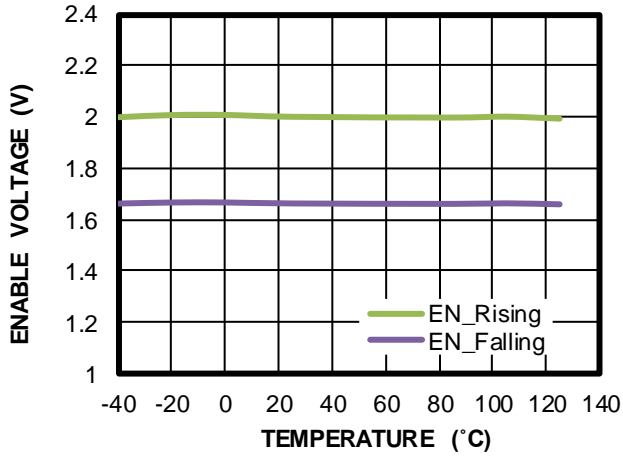
EN Rising/Falling Threshold vs. Temperature
