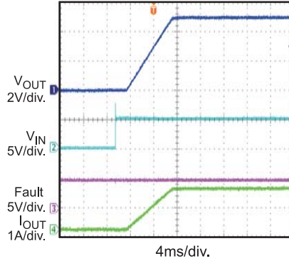
Start-Up through Input Voltage R_{LOAD} = 3.3\Omega
