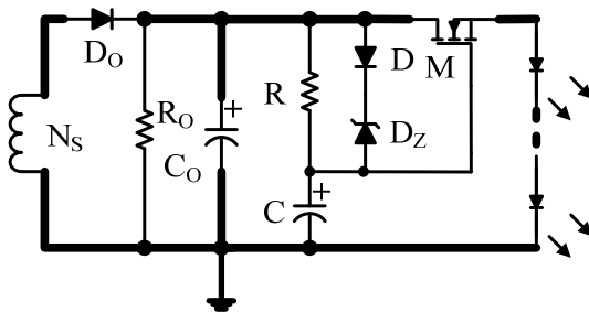
Figure9: Ripple Suppressor
