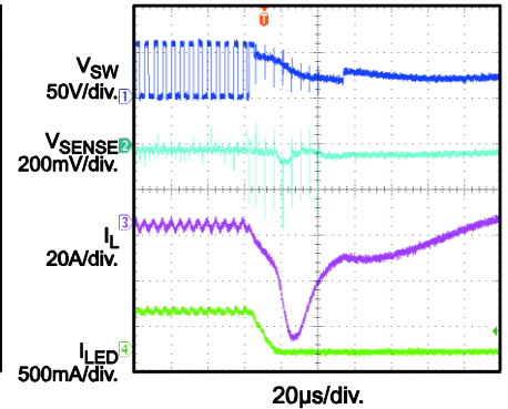
Short-Diode Protection
