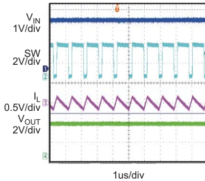
Steady Waveform
