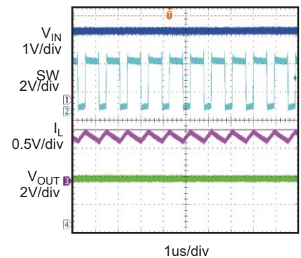
Steady Waveform
