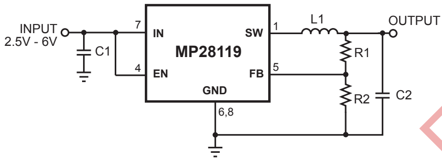
MP28119 Typical Application Circuit
