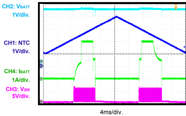
NTC Fault Indication, Charge Mode V_{IN}=5V , V_{BATT}=3.7V , R_{LIM}=71.5k\Omega , R_{SET}=71.5k\Omega
