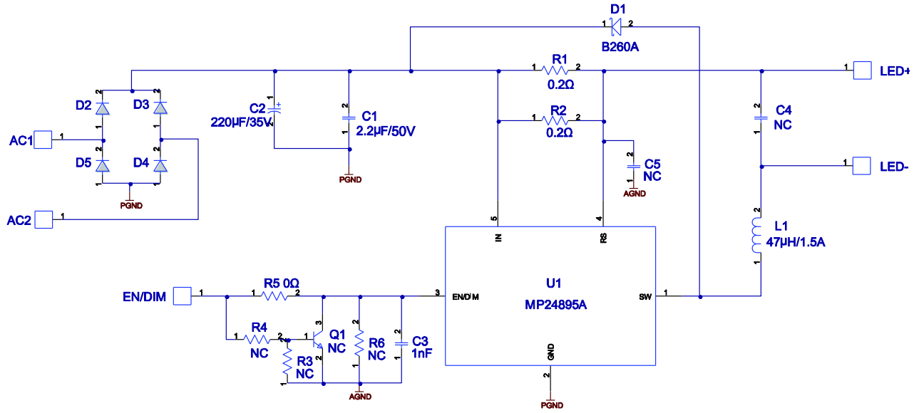
Figure 5: Drive 3 LEDs in Series, 1A Current Output
