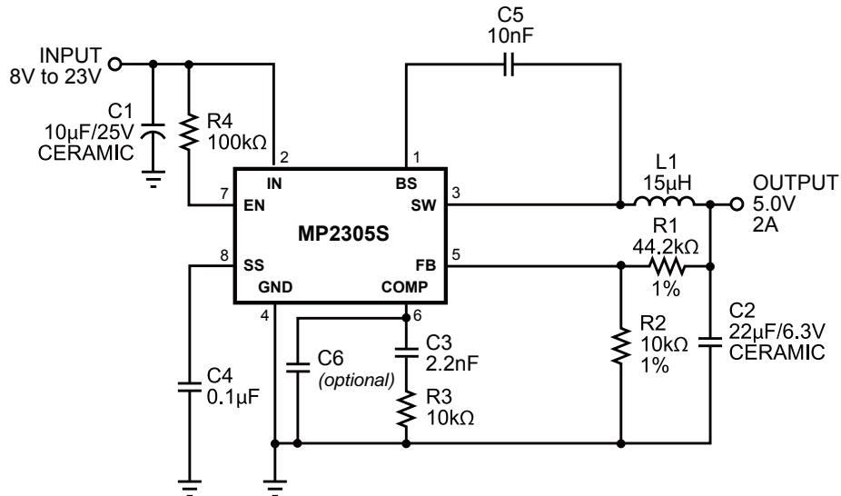
Figure 4—MP2305S with 5.0V Output, 22µF/6.3V Ceramic Output Capacitor
