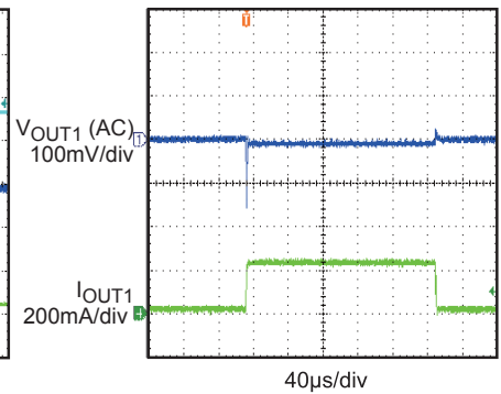
Load Transient (Ch1)
