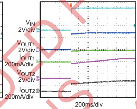
Input Power Up
