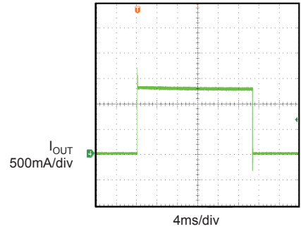
Current Limit
