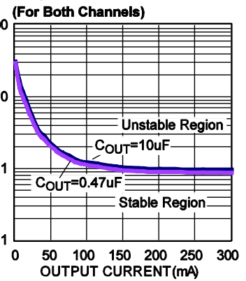
CO UT ESR Stability vs. Output Current
