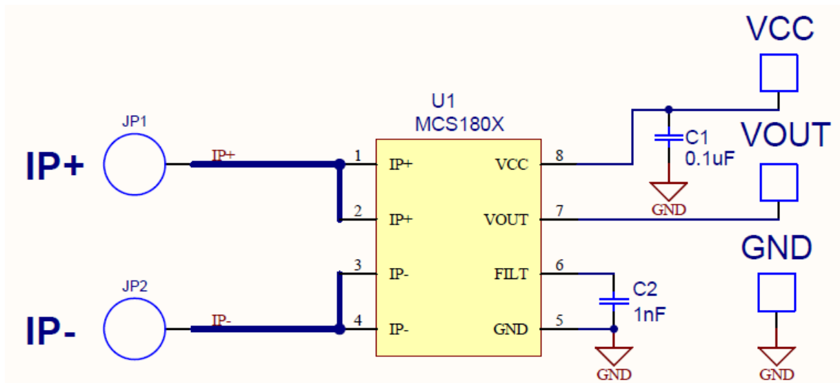
Figure 11: Application Circuit
