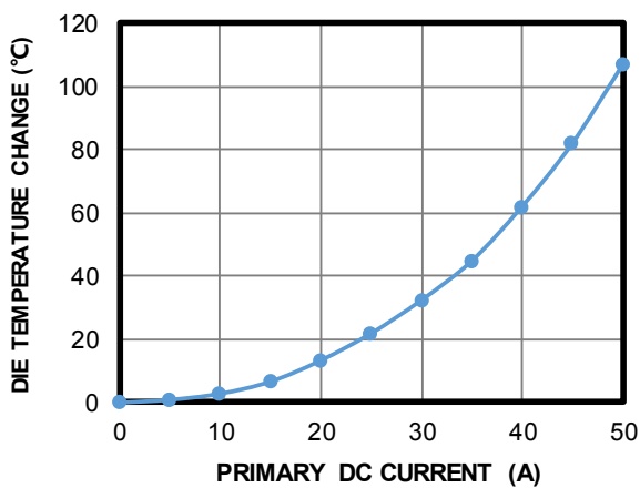
Figure 9: Self-heating Performance with DC Current Input
