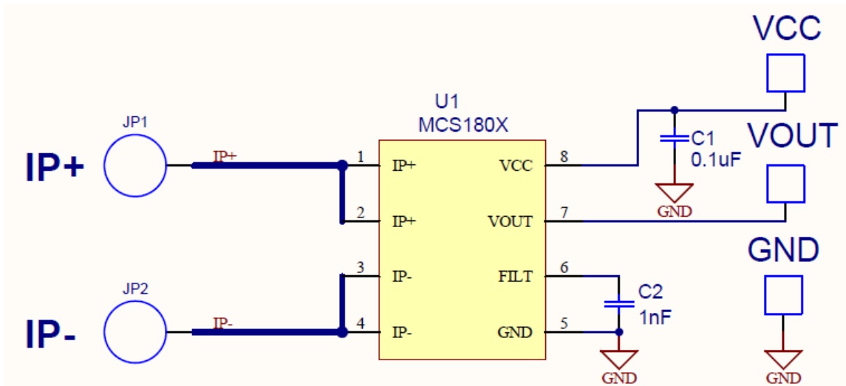
Figure 11: Application Circuit
