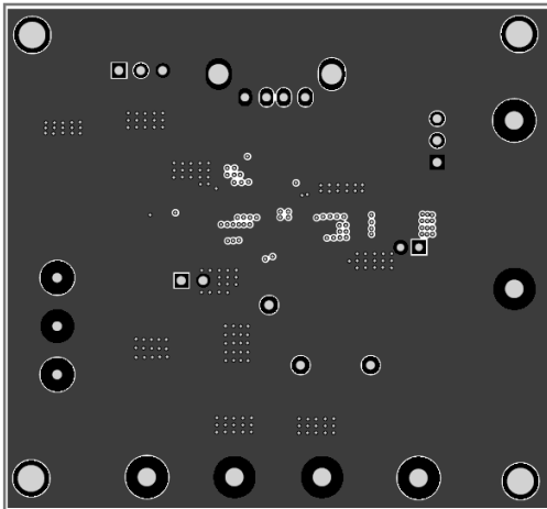
Figure 3—Mid 1 Layer
