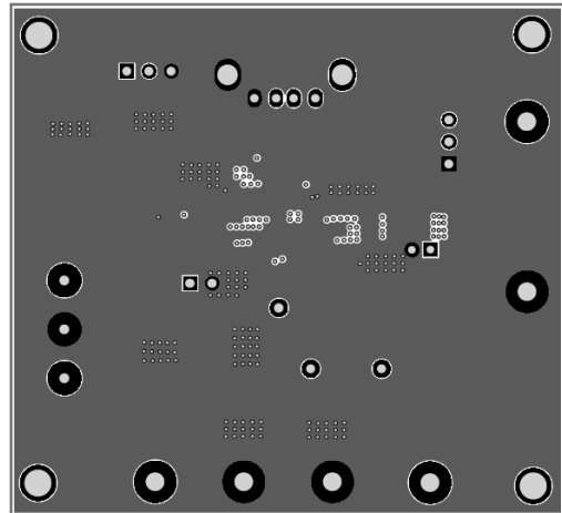
Figure 4—Mid 2 Layer
