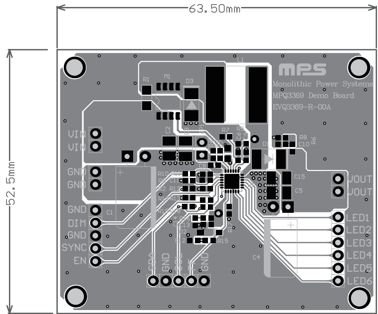
Figure 1: Top Layer
