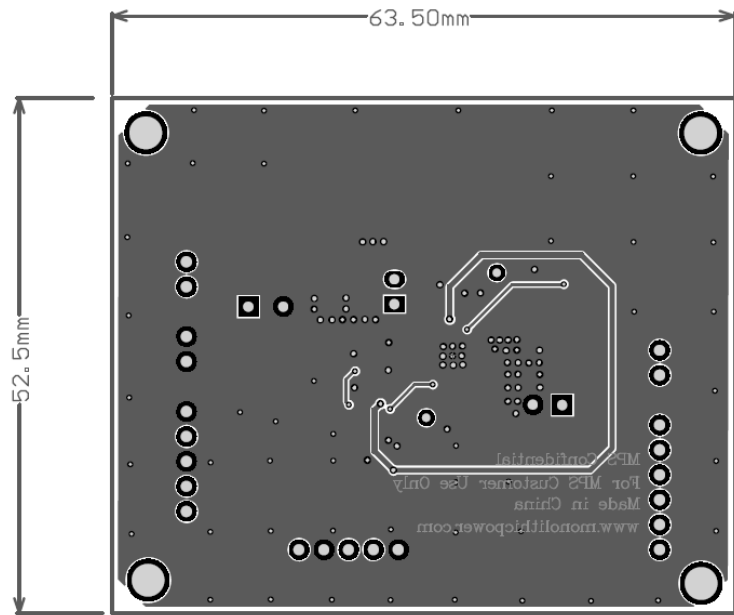
Figure 2: Bottom Layer
