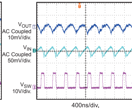
Input/Output Ripple I_{OUT} = 0.6A
