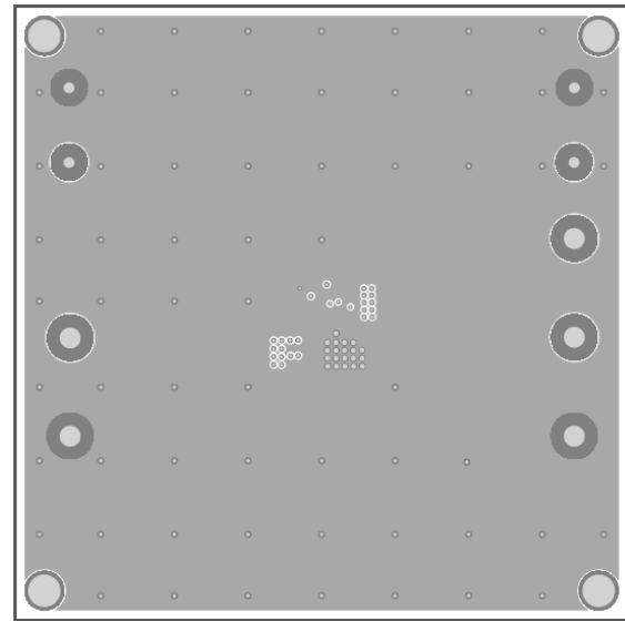
Figure 2-IN1 Layer
