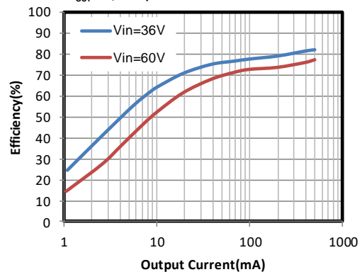
Efficiency vs. Output Current V OUT =5V, L=33µH
