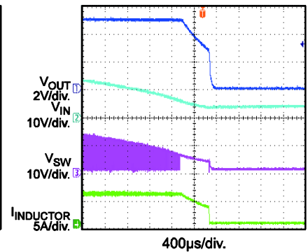
Shutdown through VIN I_{OUT} = 5A
