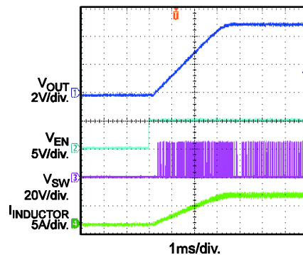
Startup through EN I_{OUT} = 5A
