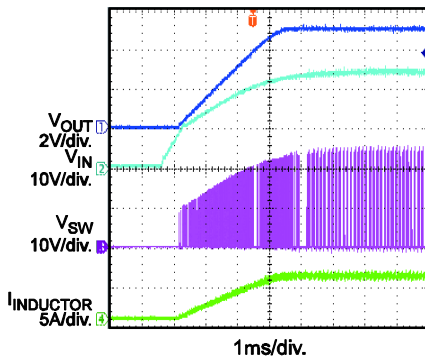
Startup through VIN I_{OUT} = 5A
