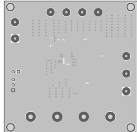
Figure 4: Inner 2 Layer
