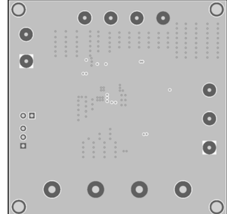
Figure 4: Inner 2 Layer
