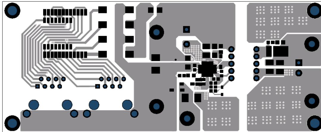
Figure 2: Top Layer
