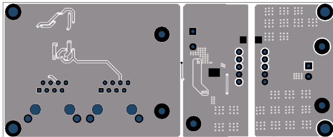
Figure 3: Bottom Layer
