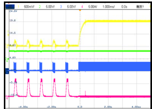
SCP Entry and Recovery SCP Recovery, no load.
