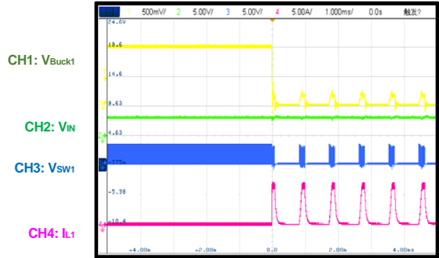
SCP Entry and Recovery SCP Entry, no load.
