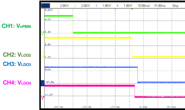
nPBIN Power off Each channel with no load
