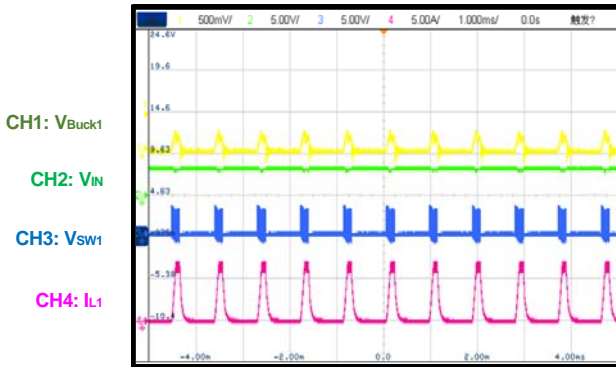
SCP Entry and Recovery SCP Steady State, no load.
