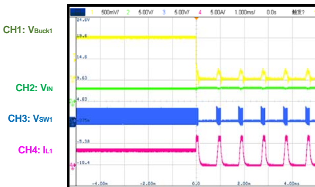
SCP Entry, full load. SCP Entry, full load.
