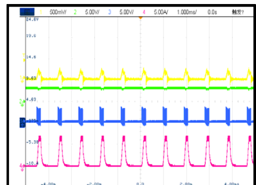
SCP Entry, full load. SCP Steady State, full load.
