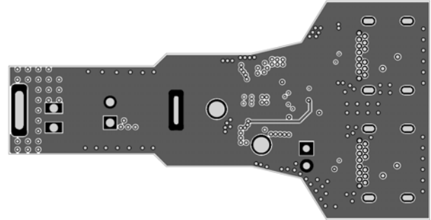
Figure 4—Middle 2 Layer
