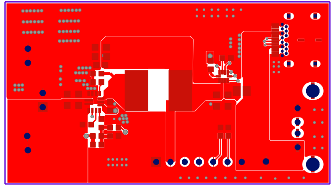
Figure 2: Top Layer
