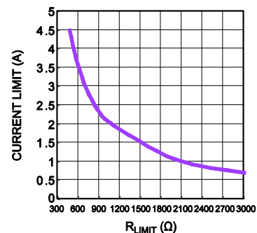
Current Limit vs. R LIMIT
