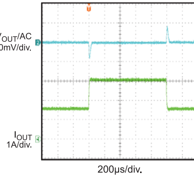
Load Transient I_{OUT} = 1.5A \leftrightarrow 3A , 1.6A/\mu s
