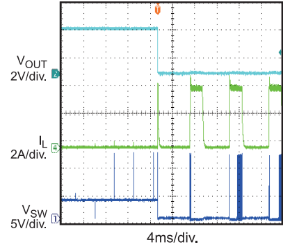
SCP Entry I_{OUT} = 0A to Short Circuit
