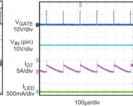
SCP steady state, LED+ short to LED-
