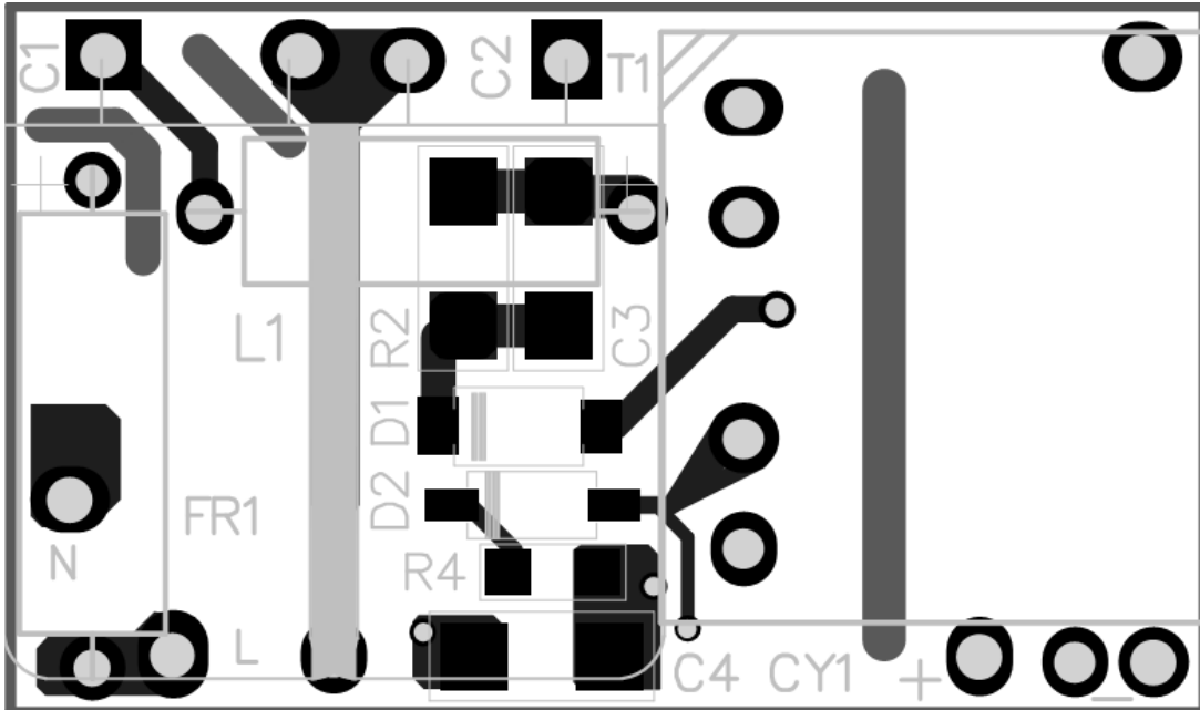
Figure 2: Top Layer
