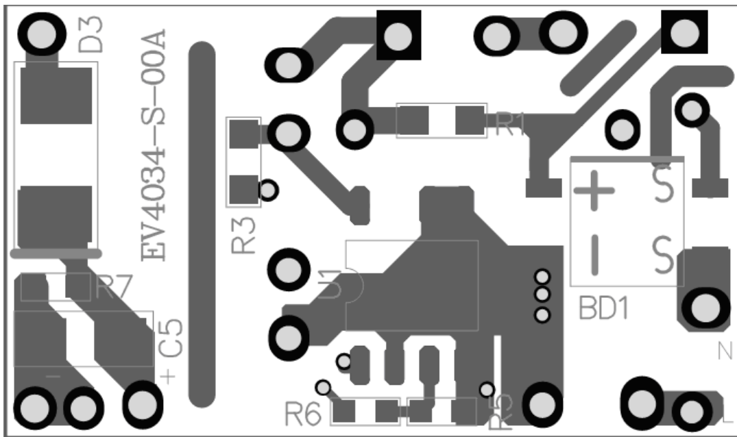
Figure 3: Bottom Layer
