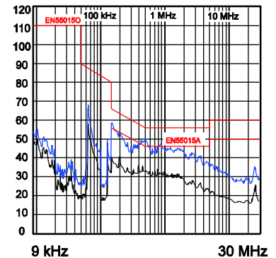
Conduction EMI
