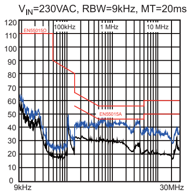
Conduction EMI
