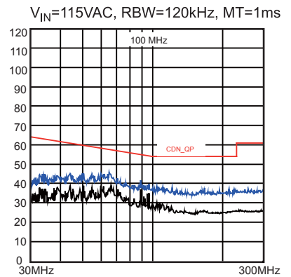
CDN Test
