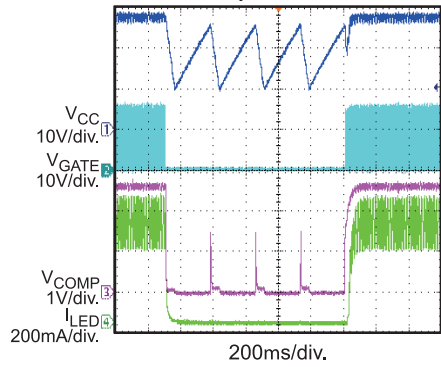
Primary-side OCP
