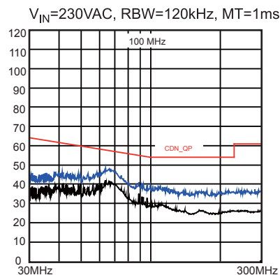
CDN Test
