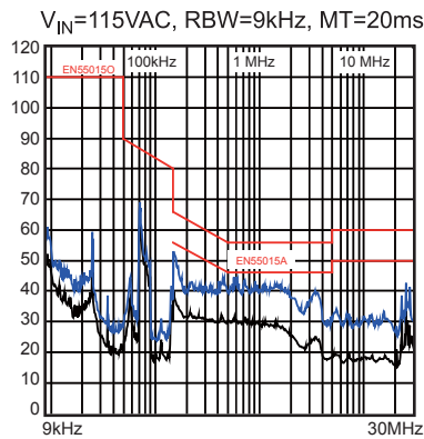
Conduction EMI
